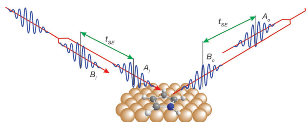
Figure 1. Schematic diagram of the HeSE experiment. The incident wavepacket is split and the two components, A_i and B_i , are separated so that they interrogate the surface with a time difference, t_{SE} . The lateral displacement of the components is shown for illustrative purposes only. The outgoing waves differ as a result of any motion occurring on the surface during t_{SE} . In this example, the outgoing component, A_o , is unchanged while B_o is phase-shifted by \pi . When the outgoing components are recombined the interference measures the de-coherence, which can be studied as a function of t_{SE} .
